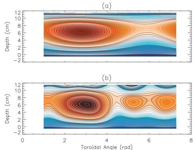
FIG. 2. (Color) Contours of toroidal flux in the reconnection ( r-\phi ) plane. (a) n=1 . (b) n=1-4 . Inclusion of n=2-4 compresses the O-point and damages the structure of the X-point. The conducting wall of MST is located along the bottom edge of the figure (depth=0).
