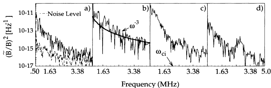
FIG. 5. Typical magnetic power spectra (a) before, (b),(c) during rise and decay, and (d) after a dynamo burst; each interval corresponds to 25 \mu s.
